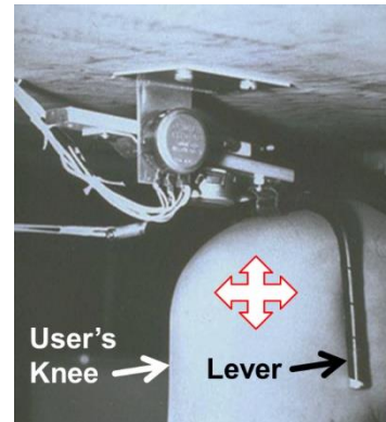
Knee-controlled lever
