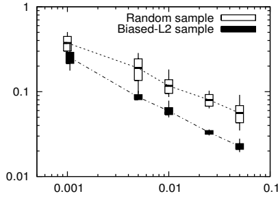
Figure 2: Log-log scale comparison of Dist_\infty(S_{Biased-L2}, D; \mathcal{H}_2) vs. Dist_\infty(S_{SRS}, D; \mathcal{H}_2) for random D of size n = 10000 , and various values of r = \alpha n (as a function of \alpha ).
