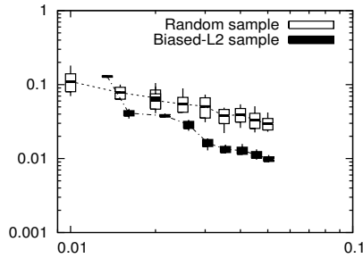
Figure 3: Log-log scale comparison of Dist_\infty(S_{Biased-L2}, D; Q_2) vs. Dist_\infty(S_{SRS}, D; Q_2) for random D of size n = 10000 , and various values of r = \alpha n (as a function of \alpha ).
